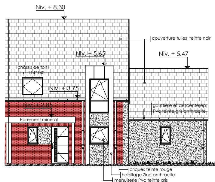
Façade Principale
